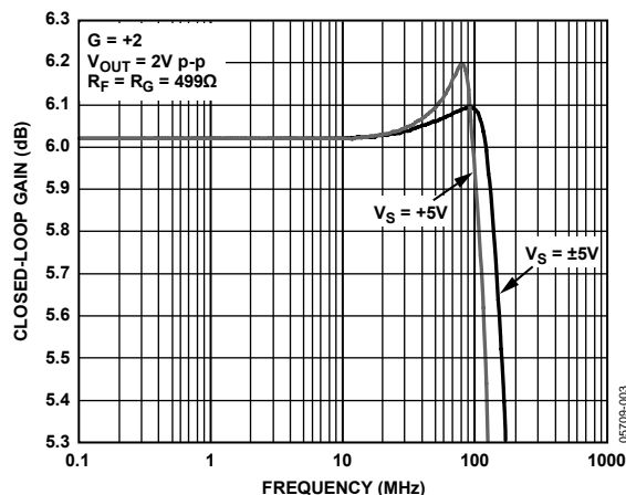
Figure 2. 0.1 dB Flatness
