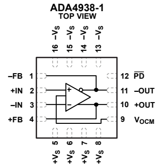
Figure 1. ADA4938-1 Functional Block Diagram
