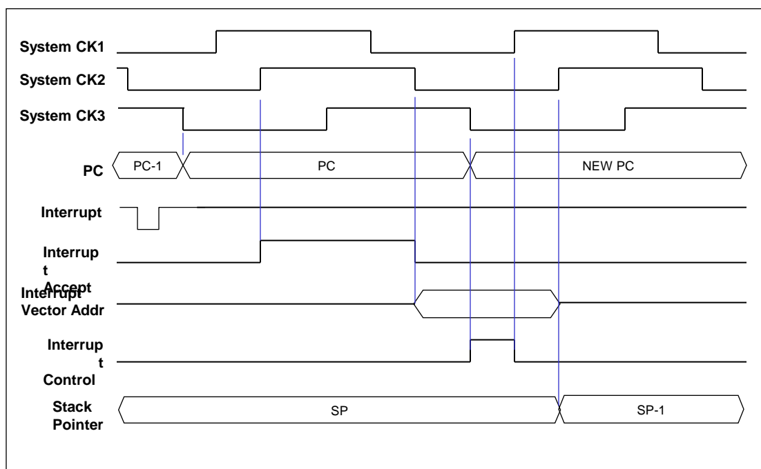
Fig. 5. 2 Interrupt Processing Step Timing
