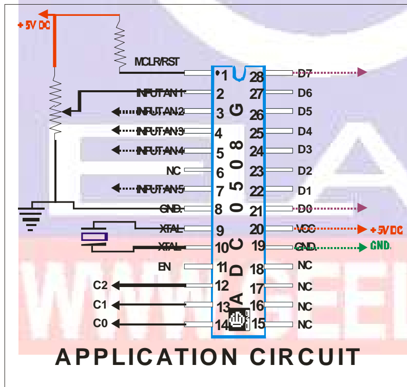
Application circuit
