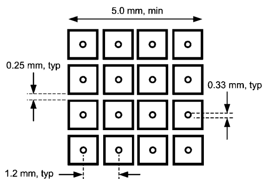
FIGURE 9. Recommended Package Land Pattern
