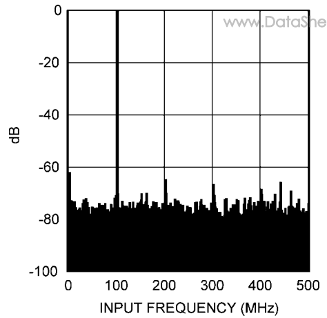
Spectral Response @ f_{IN} = 100 MHz
