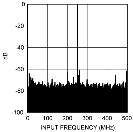
Spectral Response @ f_{IN} = 248 MHz
