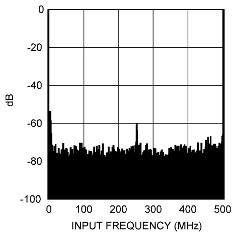
Spectral Response @ f_{IN} = 1.5 GHz
