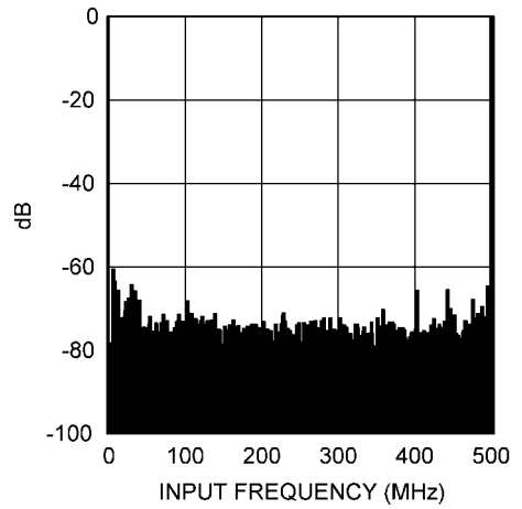
Spectral Response @ f_{IN} = 498 MHz
