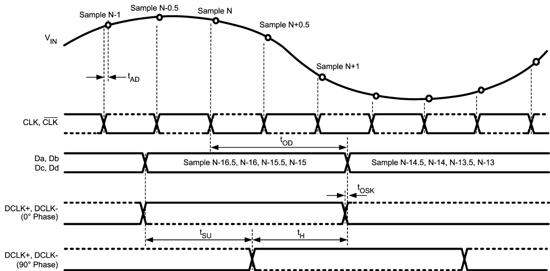
FIGURE 4. ADC082500 Timing — DDR Clocking
