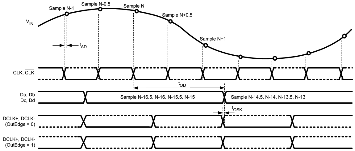
FIGURE 3. ADC082500 Timing — SDR Clocking
