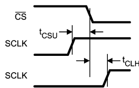
SCLK and CS Timing Parameters
