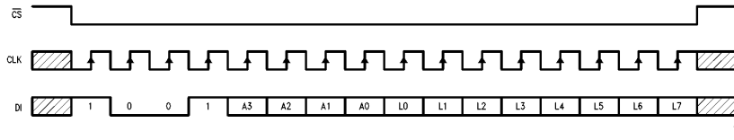
FIGURE 3. Timing Diagram for Write One Limit
