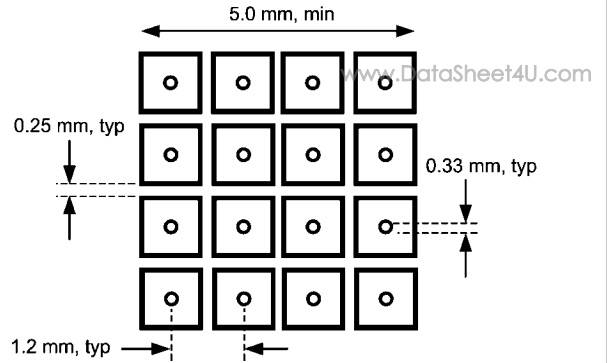
FIGURE 16. Recommended Package Land Pattern
