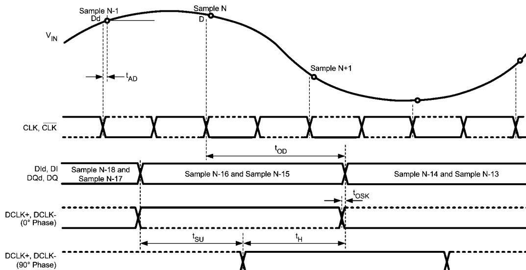
FIGURE 4. ADC08D1010 Timing — DDR Clcking
