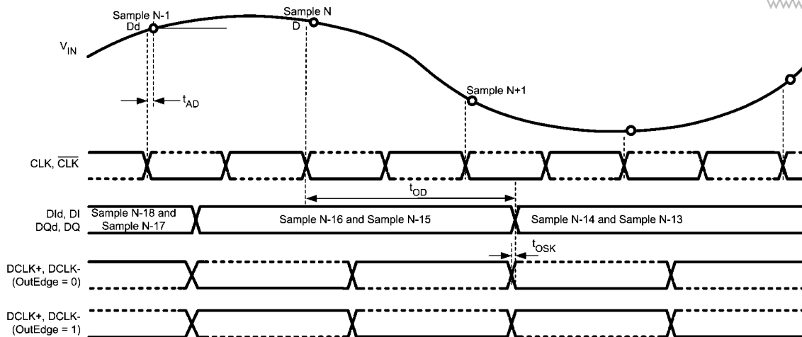
FIGURE 3. ADC08D1010 Timing — SDR Clcking
