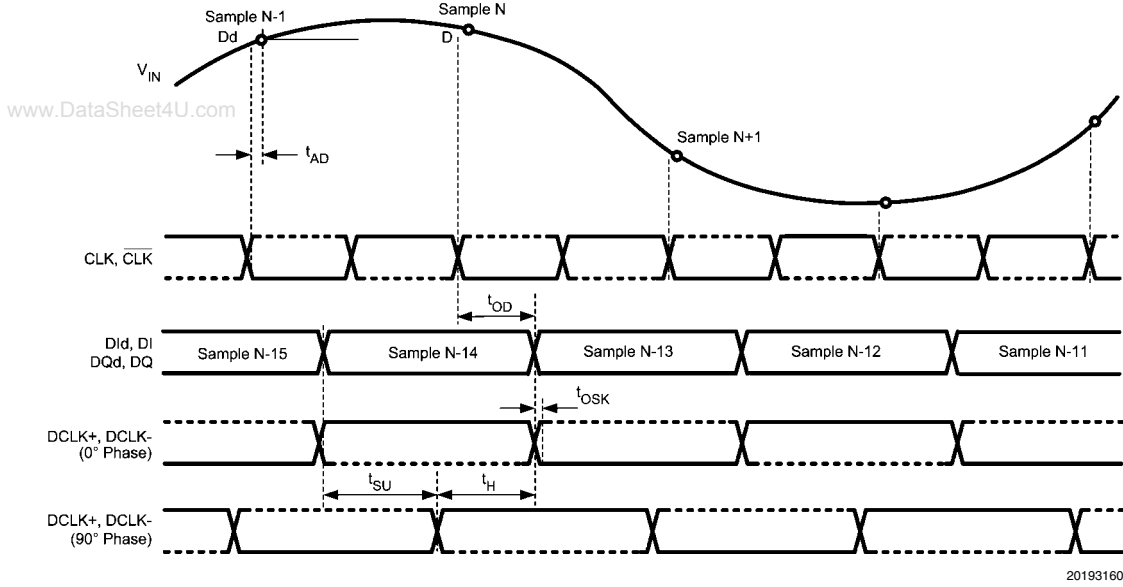
FIGURE 5. DDR Clacking in Non-Demultiplexed Non-DES Mode
