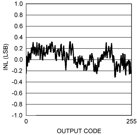
www.DataSheet4U INL vs. CODE
