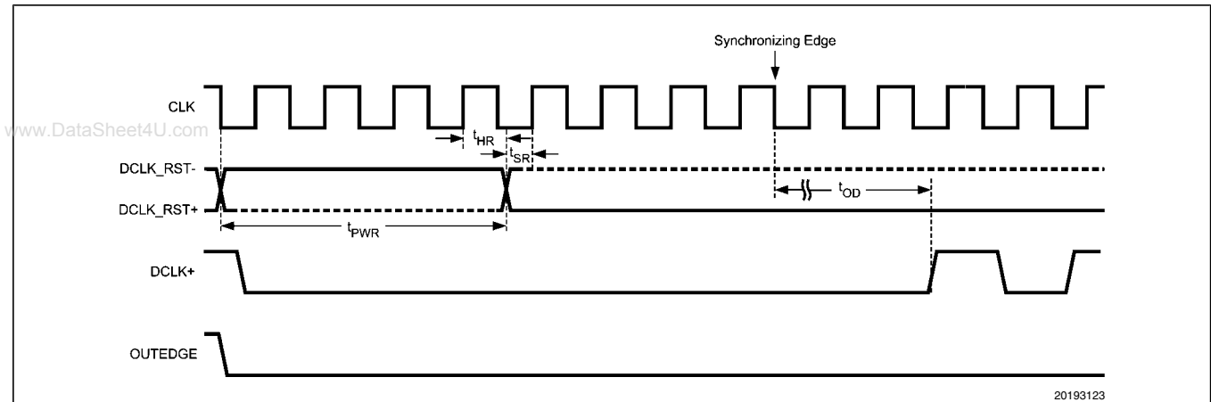
FIGURE 8. Clock Reset Timing in SDR Mode with OUTEDGE Low
