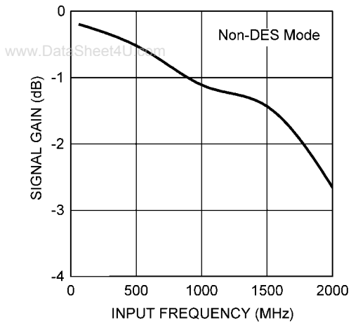
FULL POWER BANDWIDTH (NON-DES MODE)
