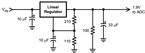
FIGURE 15. Non-Spiking Power Supply
