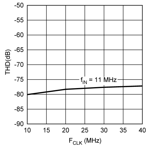
THD vs. f CLK
