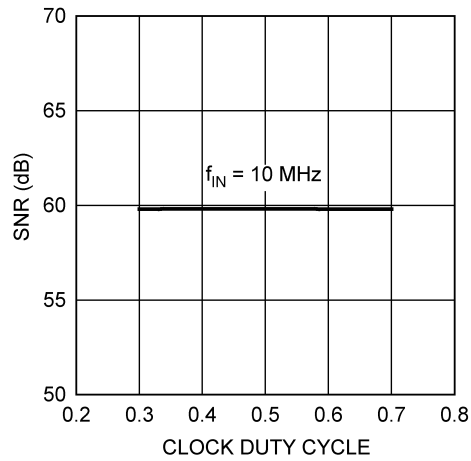
SNR vs. Clock Duty Cycle
