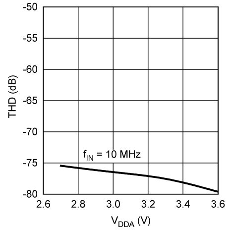
THD vs. V DDA
