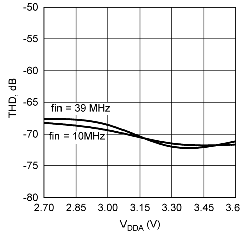
THD vs. V_{DDA}
