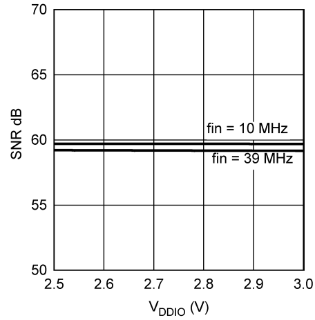
SNR vs. V_{DDIO}
