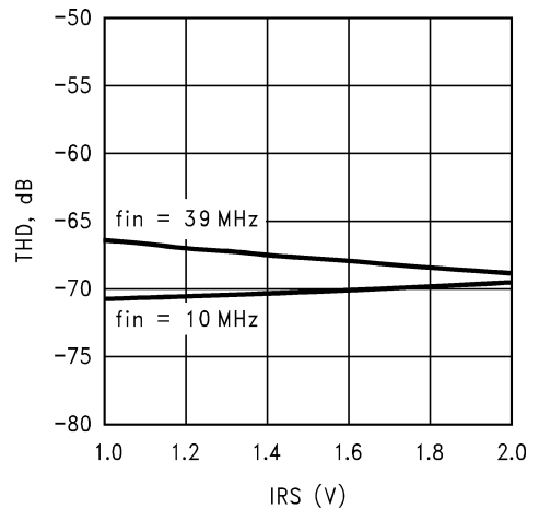
THD vs. IRS
