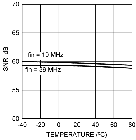
SNR vs. Temperature
