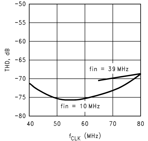
THD vs. f_{CLK}
