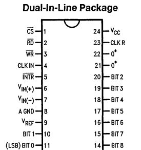
ADC1025 (10-bit parallel outputs)
