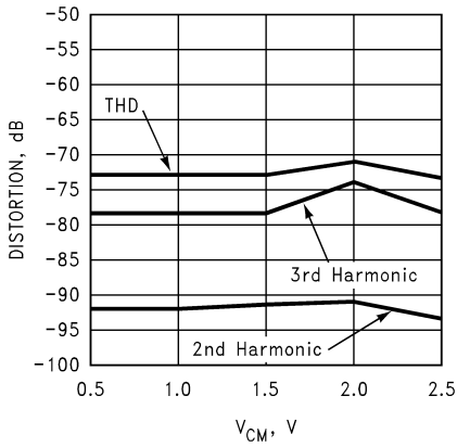
Distortion vs. V_{CM} @ f_{IN} = 4.7 MHz
