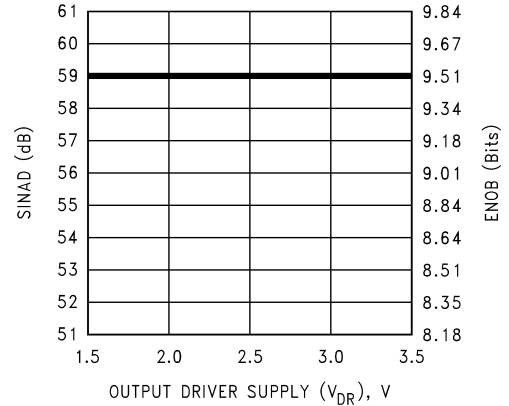
SINAD & ENOB vs. V_{DR} @ f_{IN} = 9.5 MHz
