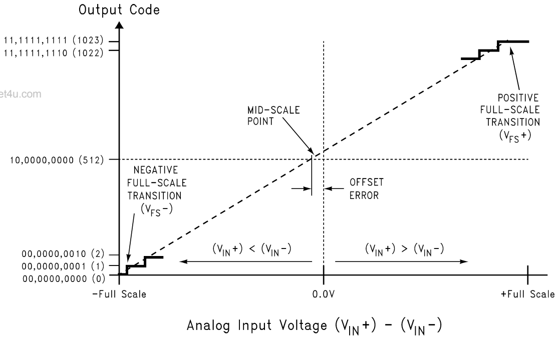
FIGURE 1. Transfer Characteristic
