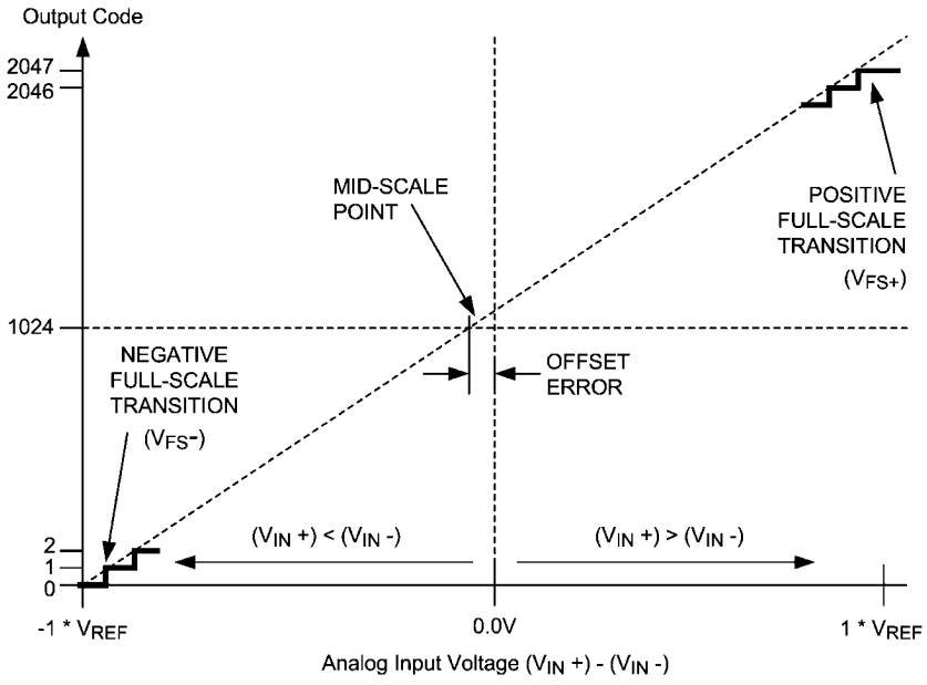
FIGURE 3. Transfer Characteristic
