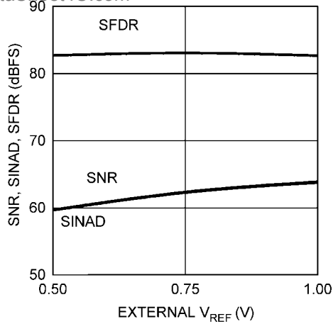
www.DataSheet4U.com SNR, SINAD, SFDR vs. Ext. Reference Voltage
