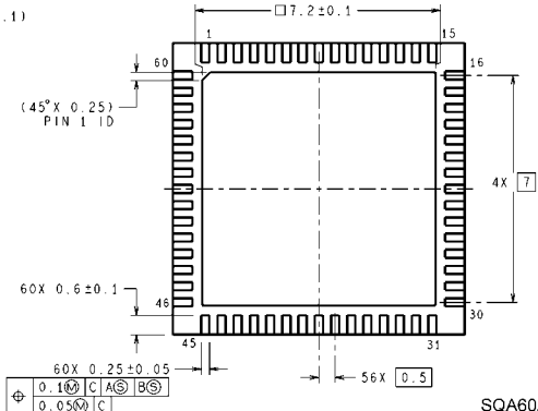
TOP View.....SIDE View.....BOTTOM View
