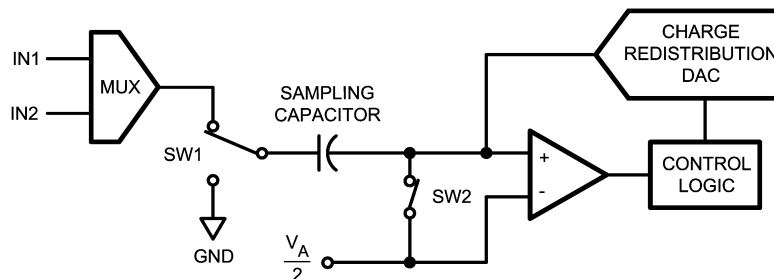
FIGURE 1. ADC122S051 in Track Mode
