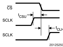
SCLK and CS Timing Parameters
