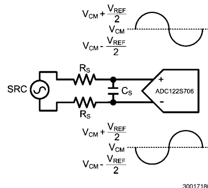
FIGURE 8. Differential Input
