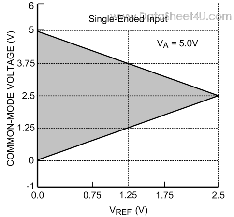
FIGURE 11. V_{CM} range for single-ended operation
