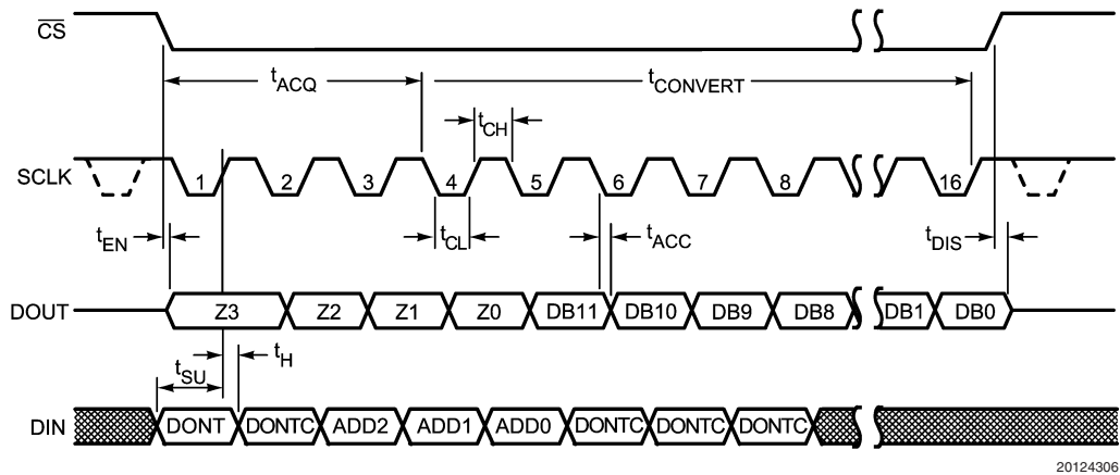
ADC124S021 Serial Timing Diagram
