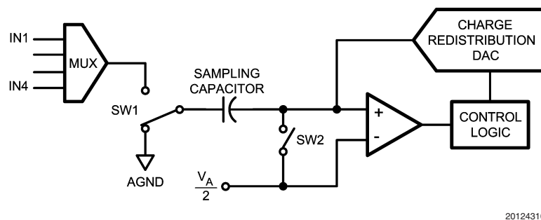
FIGURE 2. ADC124S021 in Hold Mode
