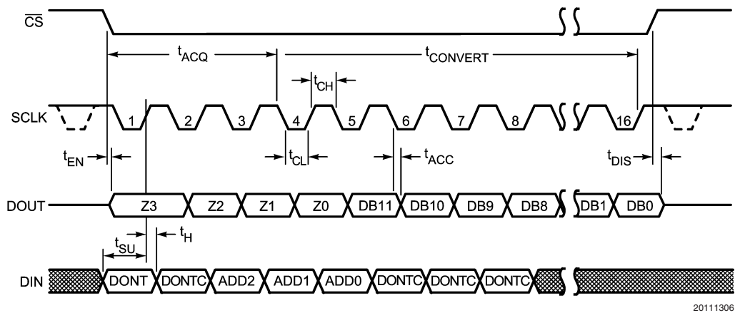
ADC124S051 Serial Timing Diagram
