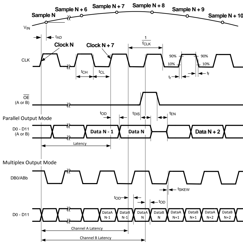
Figure 3. Output Timing
