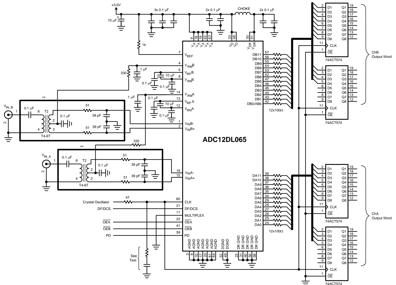
Figure 38. Application Circuit using Transformer or Differential Op-Amp Drive Circuit, Parallel mode
