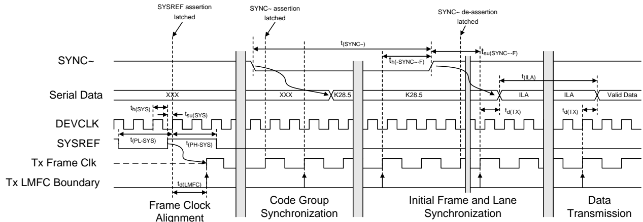
Figure 1. JESD204 Synchronization
