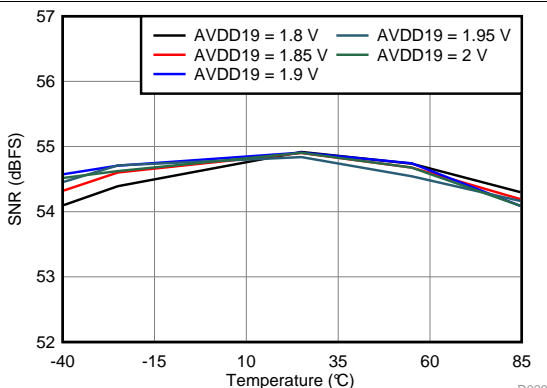
Figure 29. Signal-to-Noise Ratio vs AVDD19 Supply and Temperature
