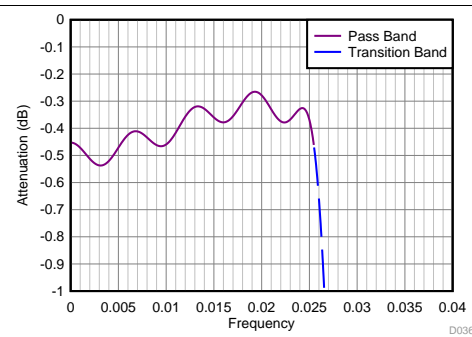
Figure 89. Divide-by-16 Filter Response (Zoomed)
