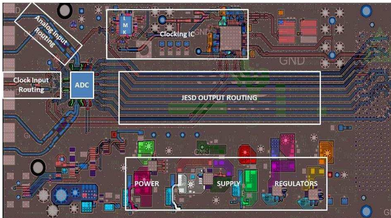
Figure 244. ADC32RF44EVM Layout
