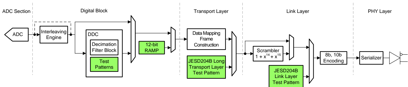
Figure 109. Test Pattern Generator Implementation
