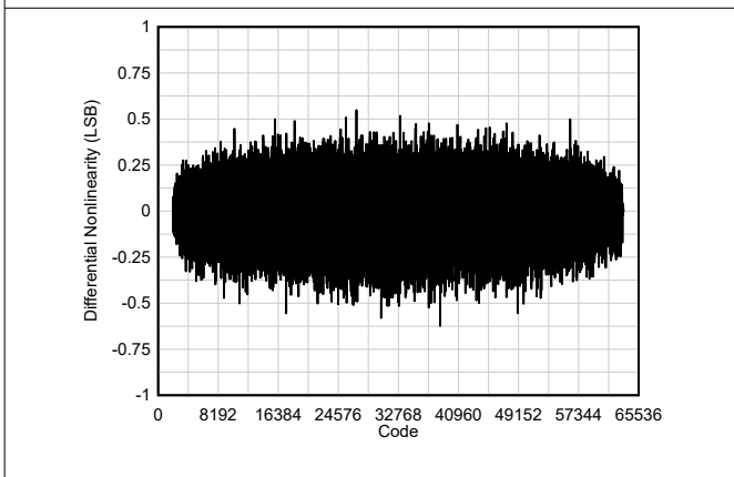
Figure 6-23. DNL
