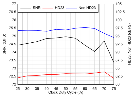
Figure 6-45. AC Performance vs Clock Duty Cycle
