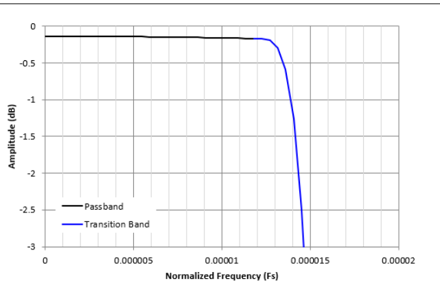
Figure 8-53. Decimation by 32768 Passband Ripple Response
