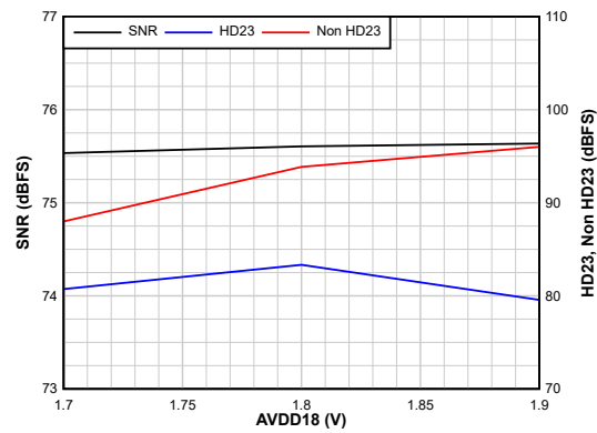
Figure 6-46. AC Performance vs AVDD18
