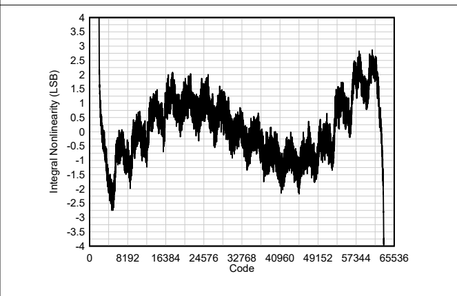
Figure 6-24. INL
