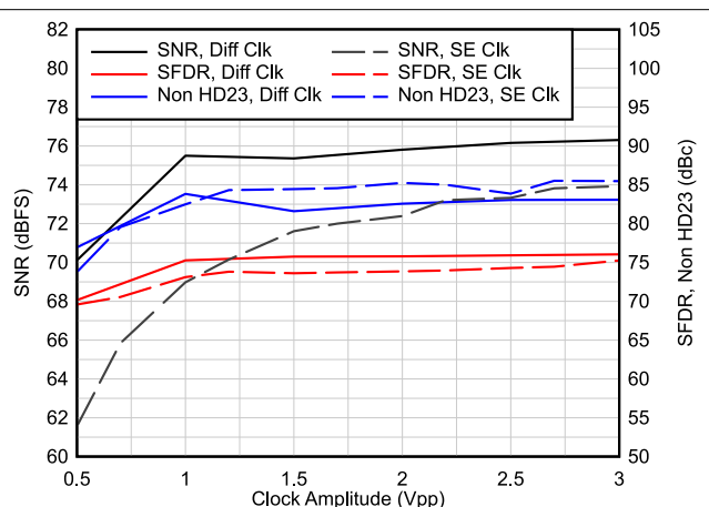
Figure 8-9. AC Performance vs Clock Amplitude for F_{IN} = 70 MHz
