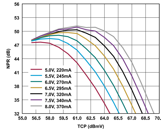
Figure 20. NPR vs. TCP Over V_{DD} and I_{DD} , Worst Case Frequency, 10 dB Tilt, R_{BIAS} = 75\ \Omega
