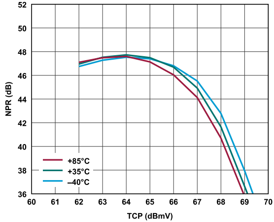
Figure 15. NPR vs. TCP Over Temperature, Worst Case Frequency, 0 dB Tilt, V_{DD} = 8.0\text{ V}
