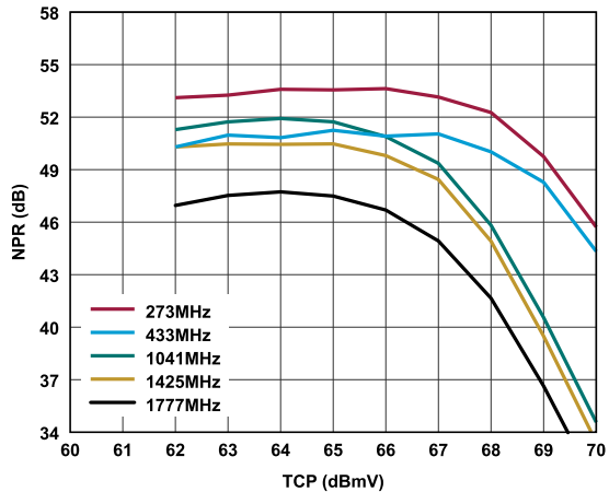
Figure 16. NPR vs. TCP Over Frequency, 0 dB Tilt, V_{DD} = 8.0\text{ V}
