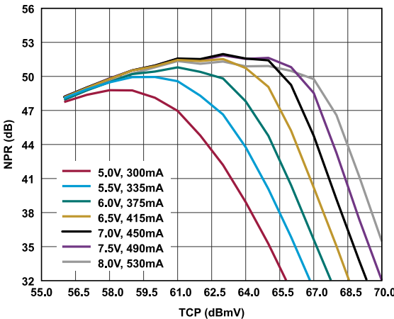
Figure 17. NPR vs. TCP Over V_{DD} and I_{DD} , Worst Case Frequency, 10 dB Tilt, R_{BIAS} = 16\ \Omega
