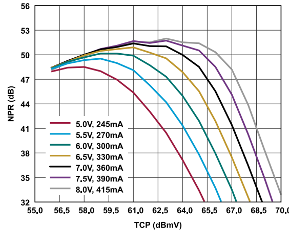
Figure 19. NPR vs. TCP Over V_{DD} and I_{DD} , Worst Case Frequency, 10 dB Tilt, R_{BIAS} = 50\ \Omega
