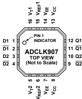
Figure 5. ADCLK907 Pin Configuration
