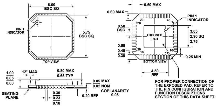
COMPLIANT TO JEDEC STANDARDS MO-220-VJJD-2 Figure 23. 40-Lead Lead Frame Chip Scale Package [LFCSP_VQ] 6 mm × 6 mm Body, Very Thin Quad (CP-40-8) Dimensions shown in millimeters
