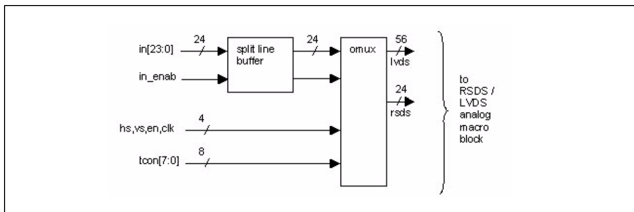
Figure 19: OMUX Architecture
