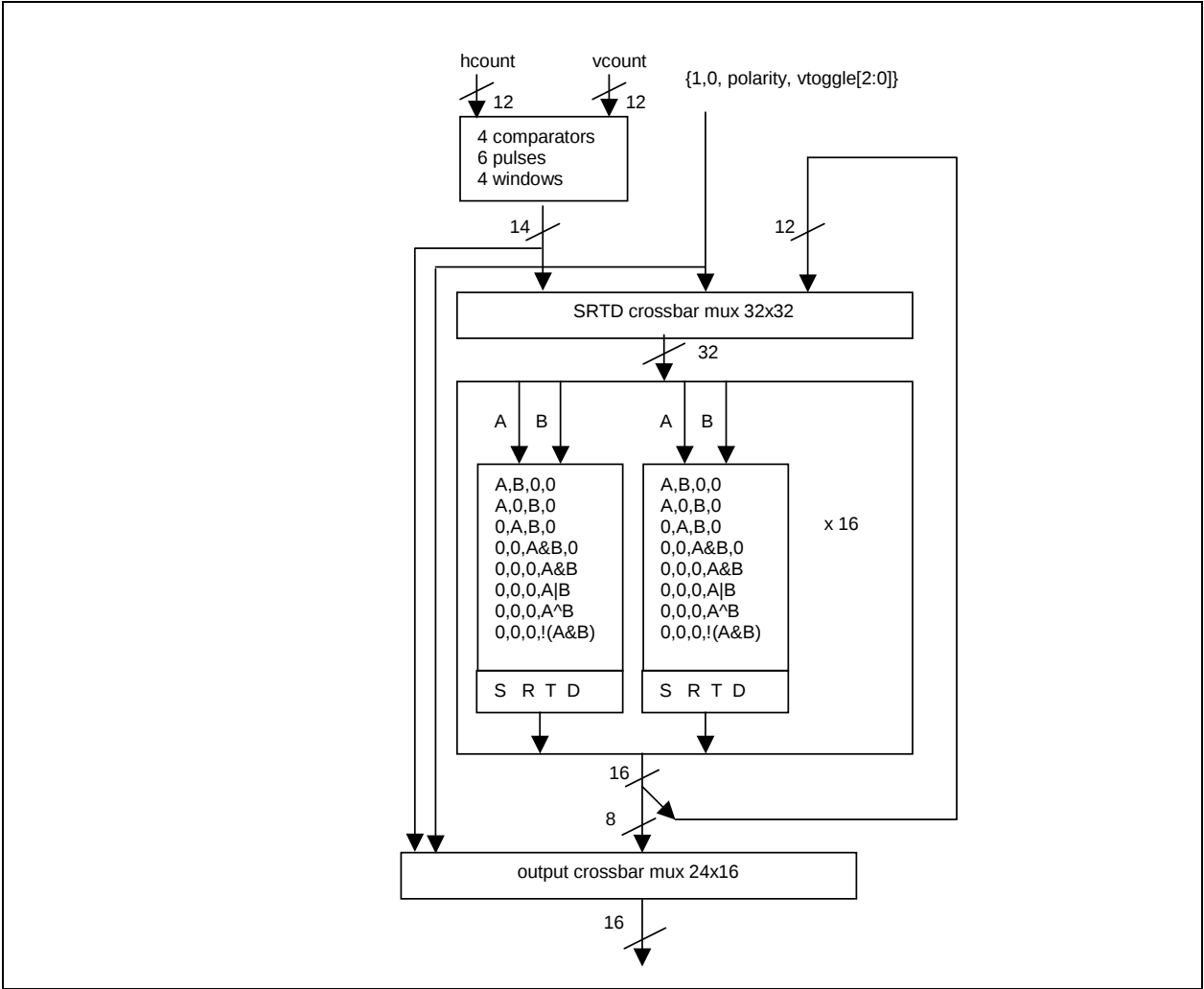
Figure 22: TCON schematic www.DataSheet4U.com
