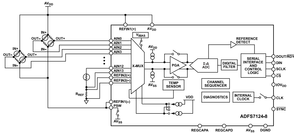
Figure 128. Flowmeter Application
