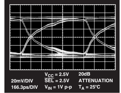
TPC 21. Eye Pattern; 1 Gbps, V_{CC} = 2.5 V , PRBS 31
