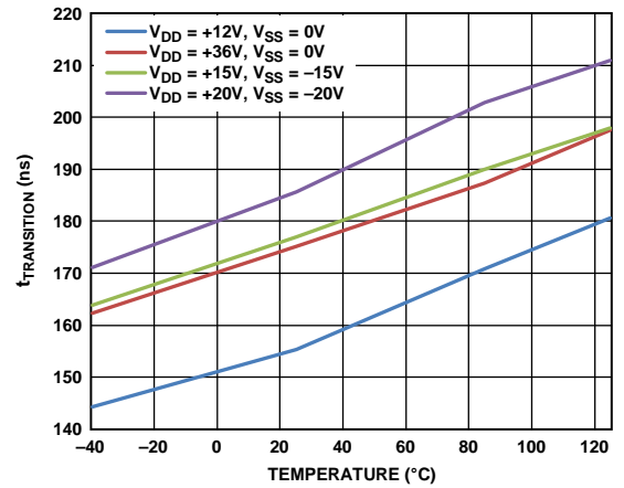
Figure 25. t_{TRANSITION} vs. Temperature
