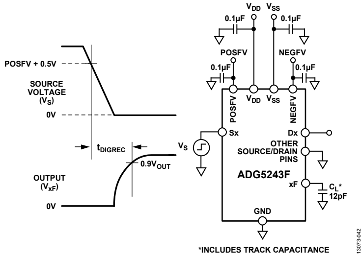
Figure 42. Interrupt Flag Recovery Time, t_{DIGREC}
