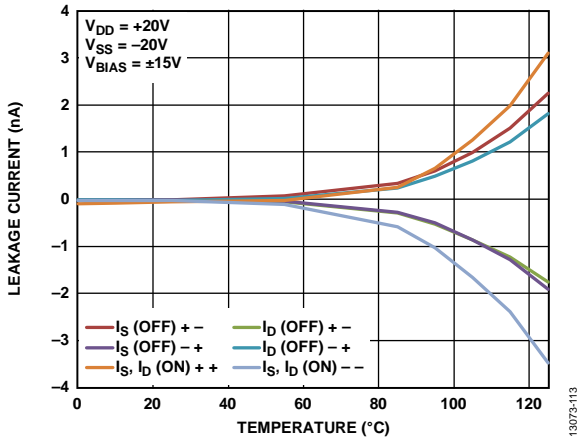
Figure 11. Leakage Current vs. Temperature, ±20 V Dual Supply
