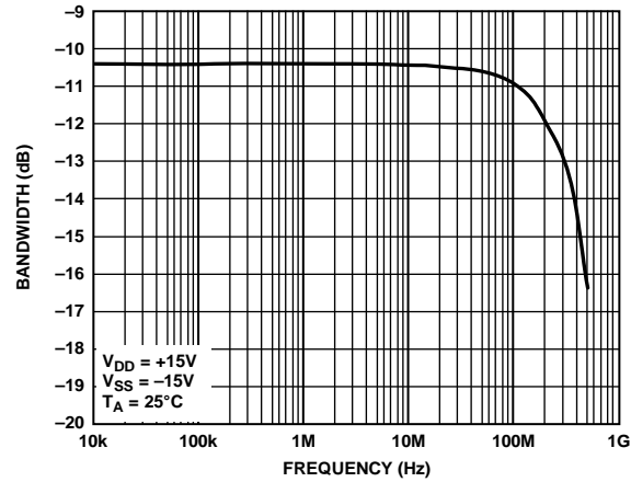
Figure 24. Bandwidth vs. Frequency
