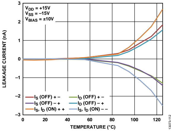
Figure 10. Leakage Current vs. Temperature, ±15 V Dual Supply
