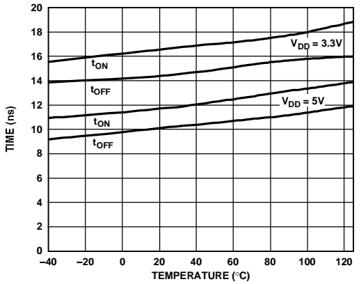
Figure 10. t_{ON}/t_{OFF} vs. Temperature
