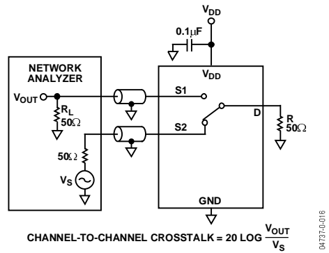
Figure 22. Channel-to-Channel Crosstalk
