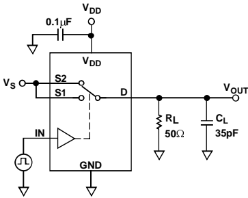
Figure 19. Break-Before-Make Time Delay, t_{BBM}
