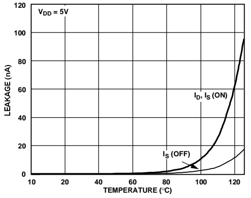
Figure 7. Leakage Currents vs. Temperature, V_{DD} = 5 V
