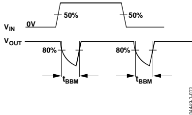
Figure 19. Break-Before-Make Time Delay, t_{BBM}
