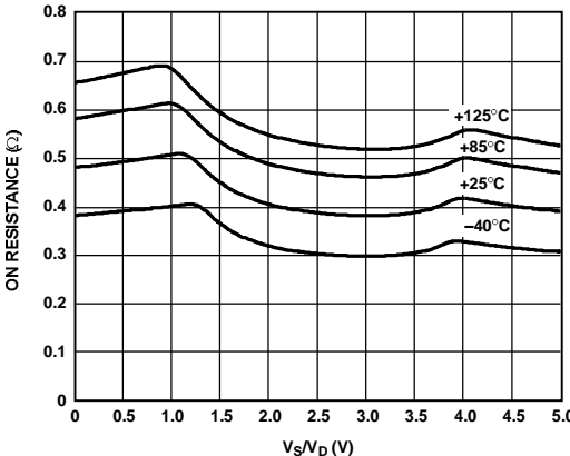
Figure 5. On-Resistance vs. Temperature, V_{DD} = 5 V
