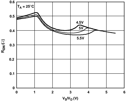
Figure 3. On-Resistance vs. V_D/V_S , V_{DD} = 5 V \pm 10\%
