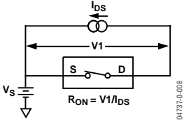
Figure 15. On-Resistance
