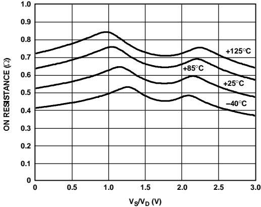
Figure 6. On-Resistance vs. Temperature, V_{DD} = 3 V
