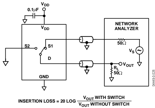
Figure 23. Bandwidth
