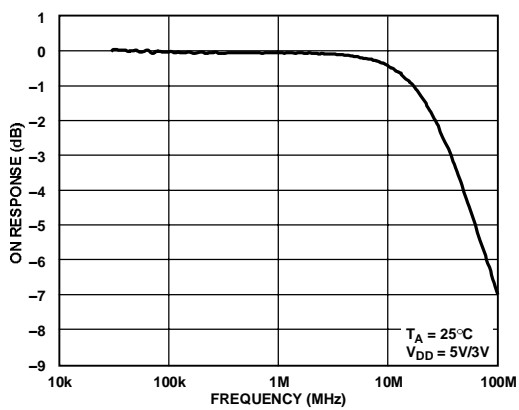
Figure 11. Bandwidth
