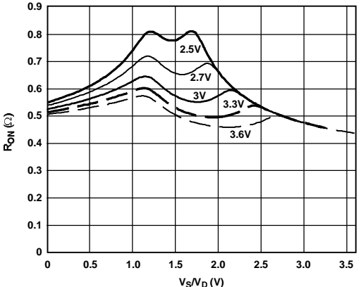
Figure 4. On-Resistance vs. V_D/V_S , V_{DD} = 2.5 V to 3.6 V
