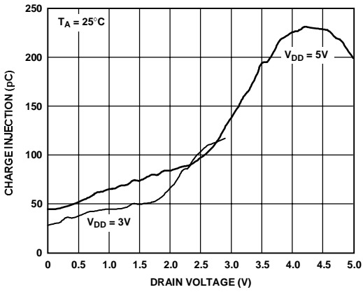
Figure 9. Charge Injection
