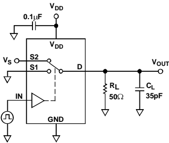
Figure 18. Switching Times, t_{ON} , t_{OFF}
