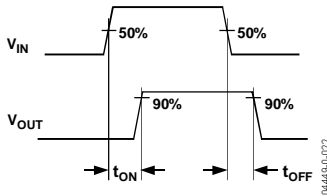
Figure 18. Switching Times, t_{ON} , t_{OFF}
