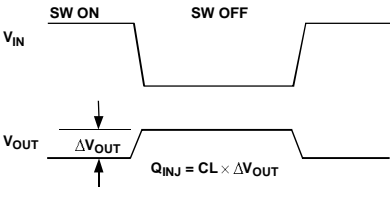
Figure 20. Charge Injection
