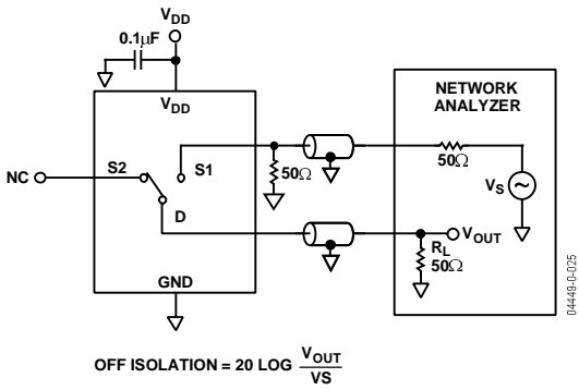
Figure 21. Off Isolation
