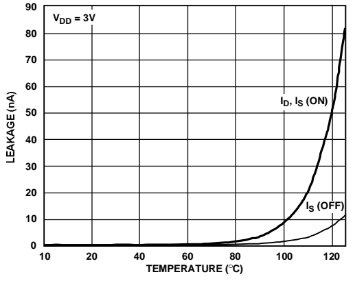
Figure 8. Leakage Currents vs. Temperature, V_{DD} = 3 V
