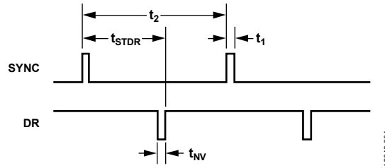
Figure 4. Input Clock Timing Diagram, Pulse Sync Mode, Register MSC_CTRL, Bits[4:2] = 101 (Binary)
