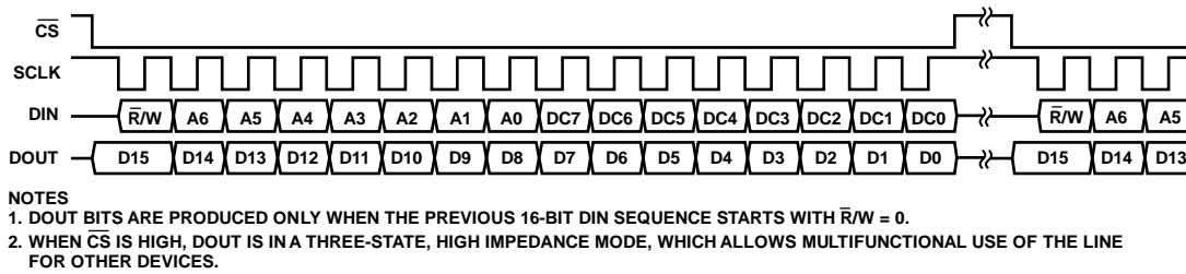
Figure 40. SPI Communication Bit Sequence
