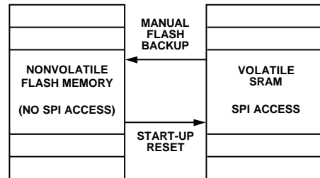
Figure 47. SRAM and Flash Memory Diagram
