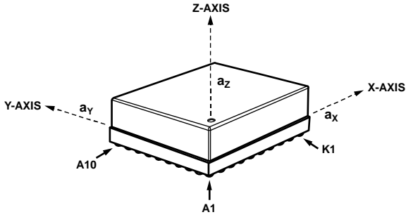
Figure 50. Accelerometer Axis and Polarity Assignments
