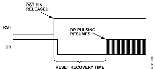
Figure 38. Data Ready Response During Reset (RST = 0) Recovery
