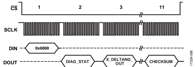
Figure 43. Burst Read Sequence with BURST_SEL = 1
