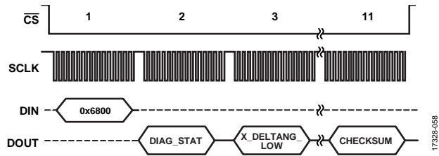
Figure 45. Burst Read Sequence with BURST_SEL = 1
