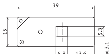
External dimensions
