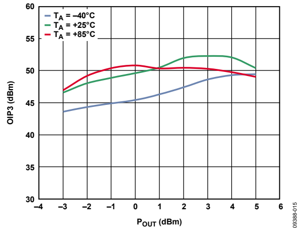
Figure 16. Output Third-Order Intercept vs. Power, Frequency = 140 MHz, Three Temperatures
