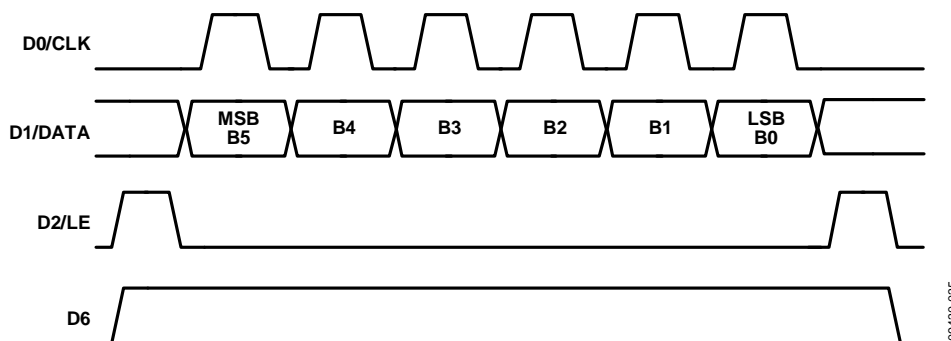
Figure 35. SPI Timing Sequence, Serial Mode
