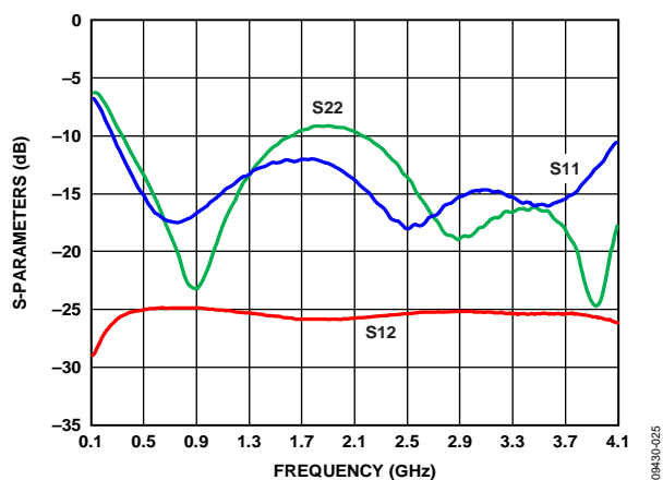
Figure 25. DSA-AMP Loop: Input Return Loss (S11), Output Return Loss (S22), and Reverse Isolation (S12) vs. Frequency, Minimum Attenuation State
