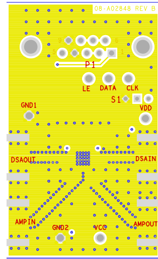
Figure 41. Evaluation Board Layout—Bottom
