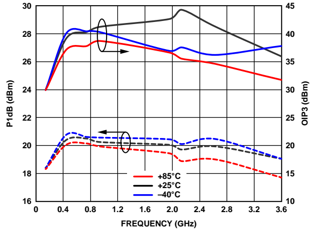
Figure 6. AMP: OIP3 at P_{OUT} = 4 \text{ dBm/Tone} and P1dB vs. Frequency and Temperature
