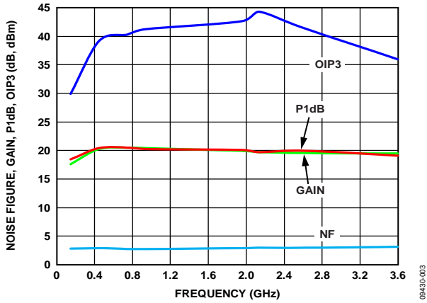
Figure 3. AMP: Gain, P1dB, OIP3 at P_{OUT} = 4 \text{ dBm/Tone} and Noise Figure vs. Frequency
