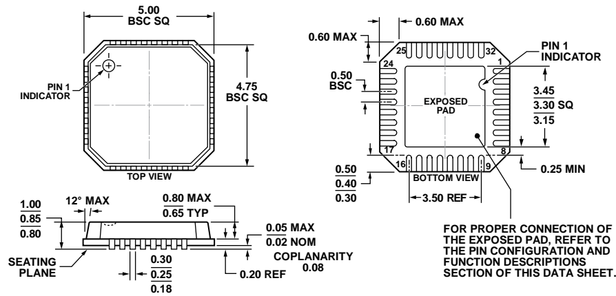
Figure 42. 32-Lead Lead Frame Chip Scale Package [LFCSP_VQ] 5 mm × 5 mm Body, Very Thin Quad (CP-32-3) Dimensions shown in millimeters
