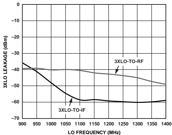
Figure 38. 3XLO Leakage vs. LO Frequency
