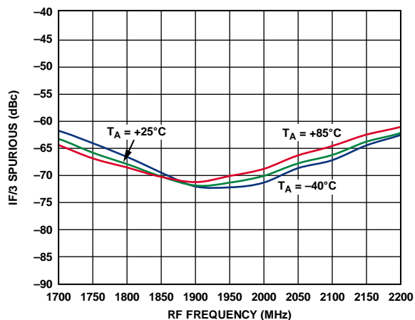
Figure 22. IF/3 Spurious vs. RF Frequency
