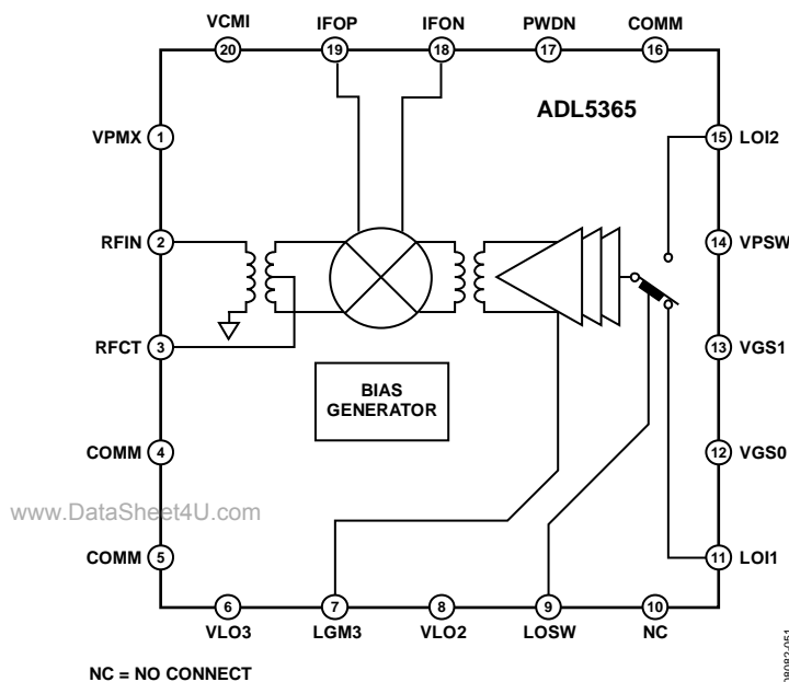
Figure 49. Simplified Schematic
