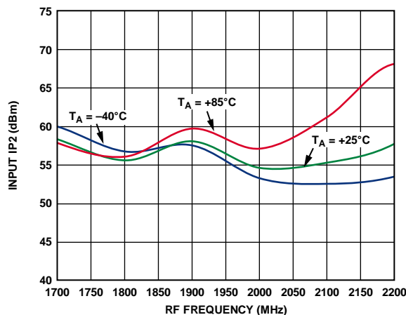
Figure 43. Input IP2 vs. RF Frequency at 3.3 V
