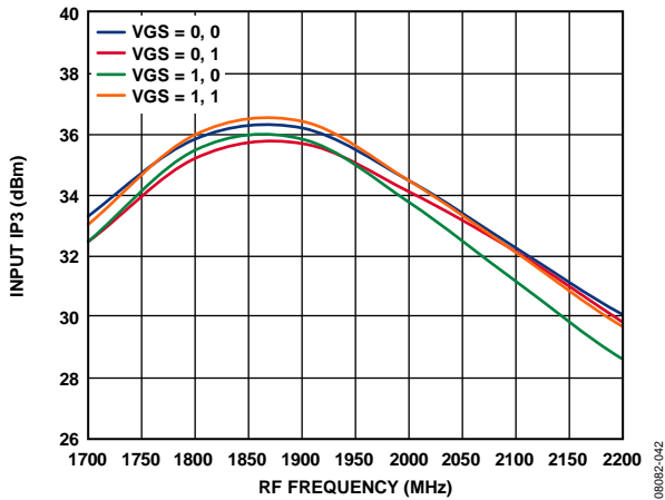
www.DataSheet4U.com Figure 36. Input IP3 vs. RF Frequency
