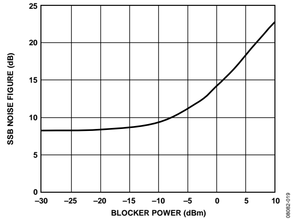
Figure 38. SSB Noise Figure vs. 10 MHz Offset Blocker Power
