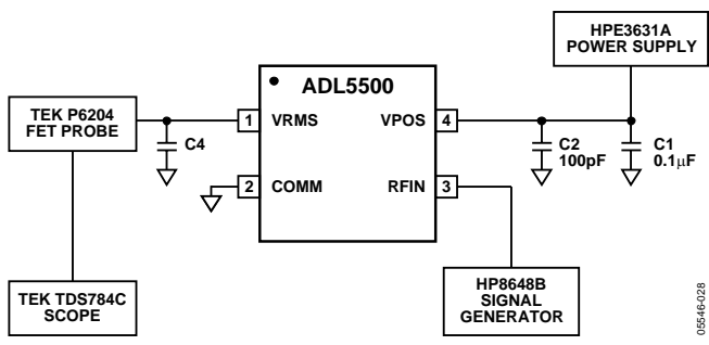
Figure 28. Hardware Configuration for Output Response to Modulated Pulse Input
