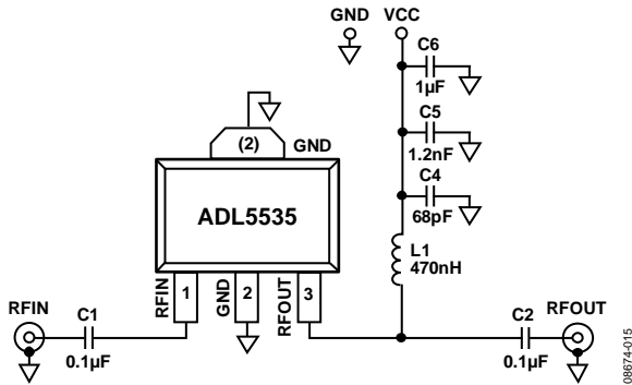
Figure 15. Basic Connections
