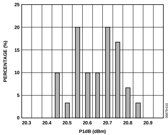
Figure 10. P1dB Distribution at 900 MHz
