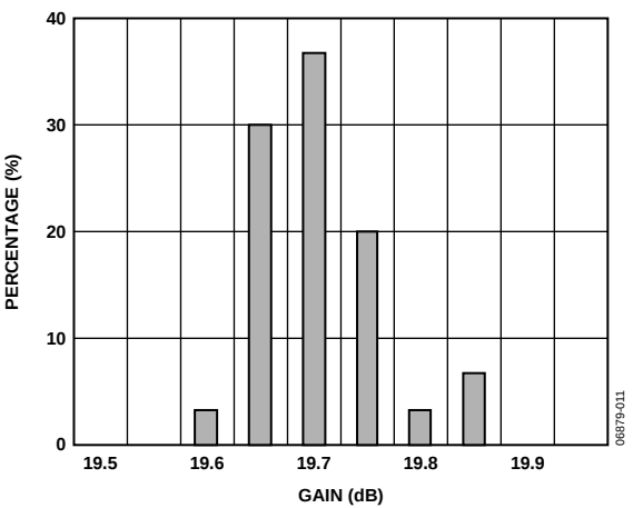
Figure 11. Gain Distribution at 900 MHz
