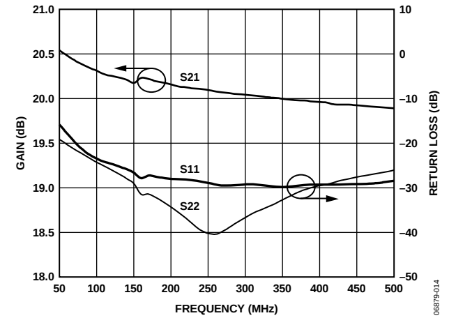
Figure 14. Input Return Loss (S11), Output Return Loss (S22), and Gain (S21) vs. Frequency
