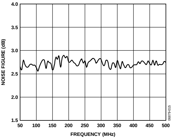
Figure 15. Noise Figure vs. Frequency
