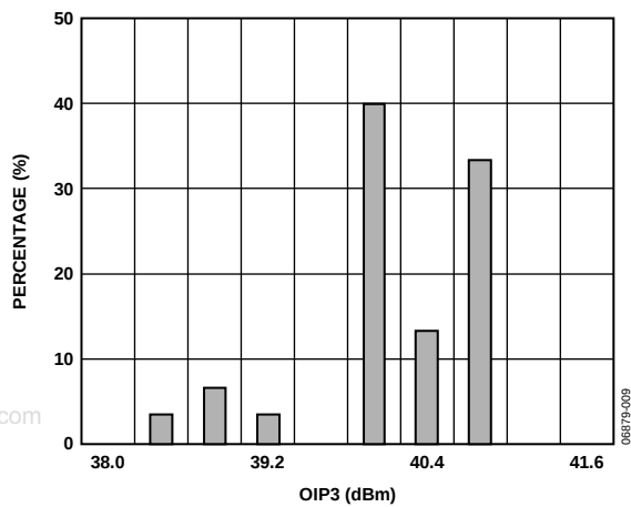
Figure 9. OIP3 Distribution at 900 MHz
