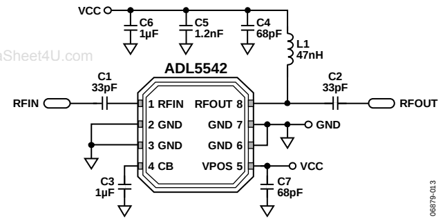
Figure 13. Basic Connections
