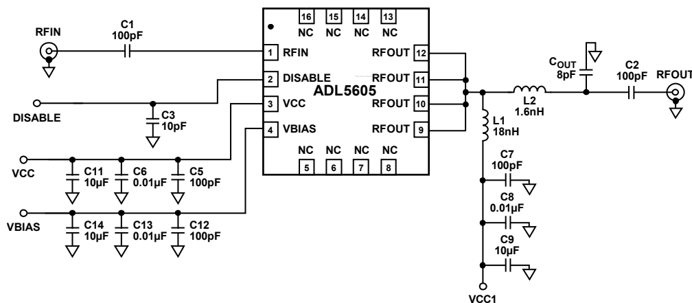
Figure 31. Basic Connections
