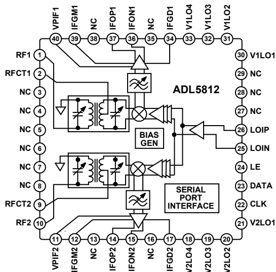
Figure 59. Simplified Schematic
