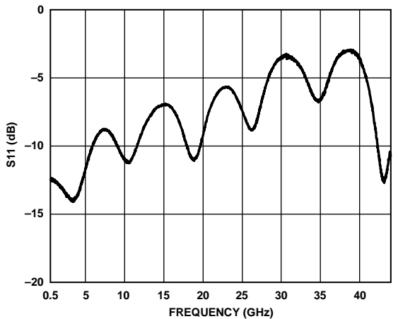
Figure 5. Input Return Loss (S 11 ) vs. Input Frequency with Input Connector and PCB Trace Embedded
