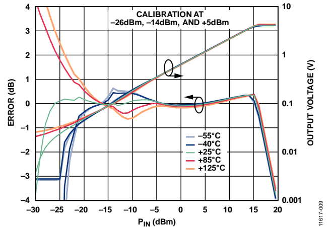
Figure 7. Conformance Error and Output Voltage (V OUT ) vs. RF Input Power (P IN ) for Various Temperatures at 0.5 GHz
