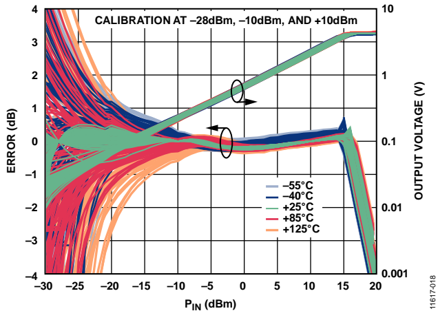
Figure 16. Distribution of Conformance Error with Respect to Output Voltage ( V_{OUT} ) at 25°C vs. RF Input Power ( P_{IN} ) for Various Temperatures at 10 GHz
