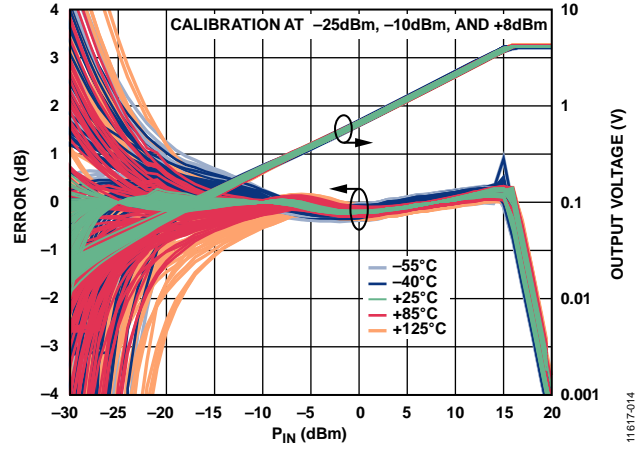
Figure 12. Distribution of Conformance Error with Respect to Output Voltage ( V_{out} ) at 25°C vs. RF Input Power ( P_{in} ) for Various Temperatures at 5 GHz
