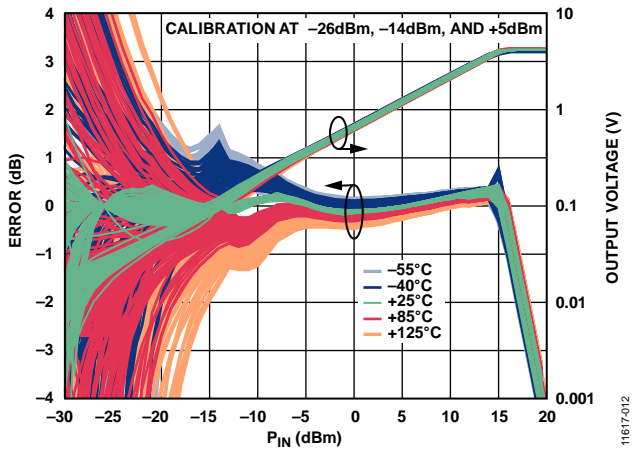
Figure 10. Distribution of Conformance Error with Respect to Output Voltage ( V_{out} ) at 25°C vs. RF Input Power ( P_{in} ) for Various Temperatures at 0.5 GHz
