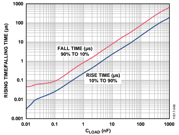
Figure 43. Rising Time/Falling Time vs. C_{LOAD} for a 1 GHz Modulated Pulsed Waveform with P_{IN} = 0 dBm
