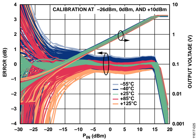
Figure 23. Distribution of Conformance Error with Respect to Output Voltage ( V_{OUT} ) at 25°C vs. RF Input Power ( P_{IN} ) for Various Temperatures at 30 GHz
