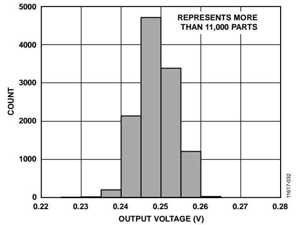
Figure 30. Output Voltage ( V_{OUT} ) Distribution, P_{IN} = -9 dBm at 12 GHz, 25°C
