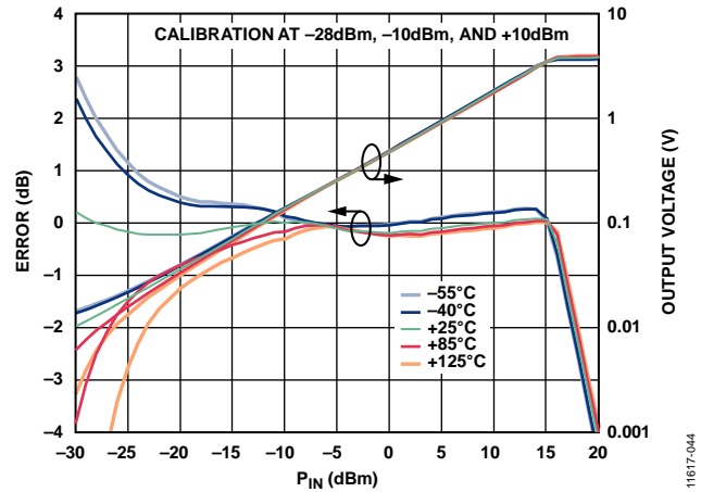
Figure 41. 10 GHz Conformance Error and Output Voltage vs. RF Input Power ( P_{IN} ) for Second Device at +25°C, -40°C, -55°C, +85°C, and +125°C
