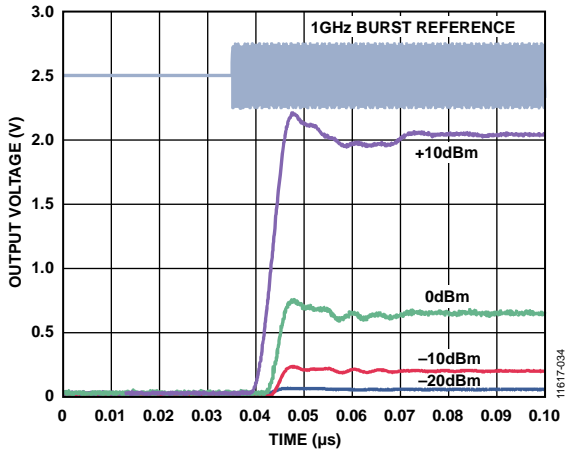
Figure 31. RF Burst Input Response, Rising Edge (see Figure 34 in the Measurement Setups Section)
