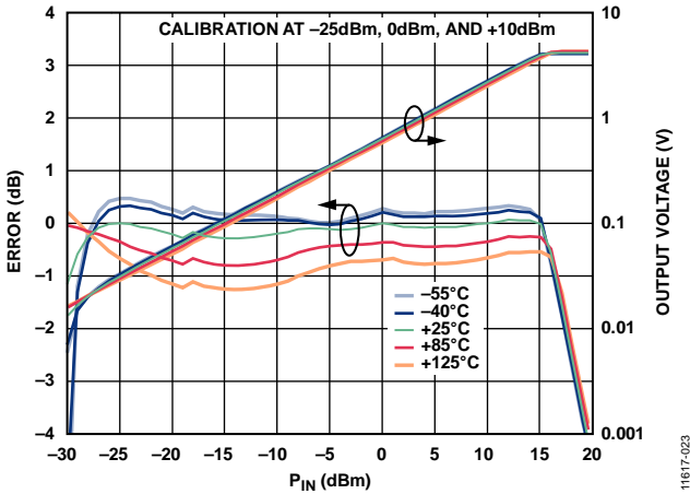
Figure 21. Conformance Error and Output Voltage ( V_{OUT} ) vs. RF Input Power ( P_{IN} ) for Various Temperatures at 35 GHz
