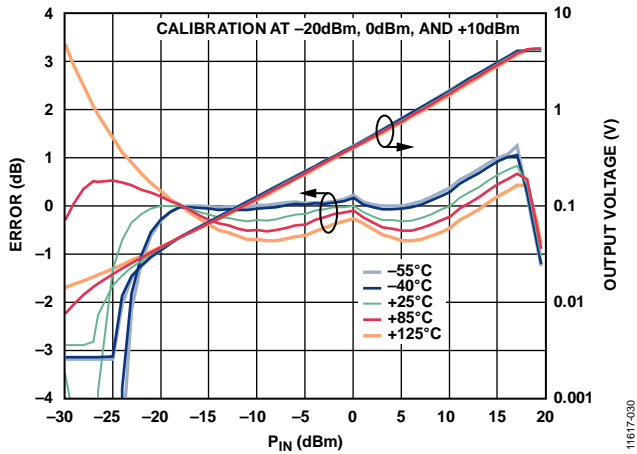
Figure 28. Conformance Error and Output Voltage ( V_{OUT} ) vs. RF Input Power ( P_{IN} ) for Various Temperatures at 43.5 GHz
