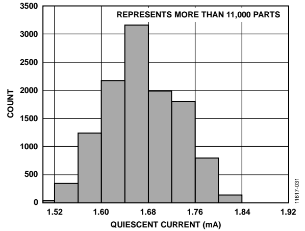
Figure 29. Distribution of Quiescent Current at 25°C
