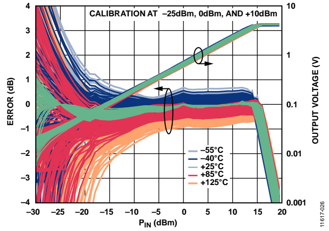
Figure 24. Distribution of Conformance Error with Respect to Output Voltage ( V_{OUT} ) at 25°C vs. RF Input Power ( P_{IN} ) for Various Temperatures at 35 GHz
