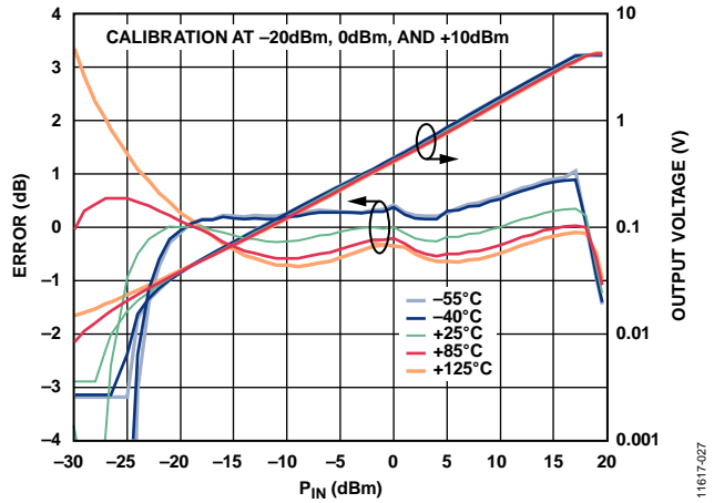
Figure 25. Conformance Error and Output Voltage ( V_{OUT} ) vs. RF Input Power ( P_{IN} ) for Various Temperatures at 40 GHz
