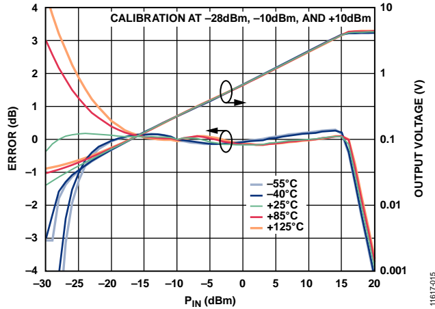
Figure 13. Conformance Error and Output Voltage ( V_{out} ) vs. RF Input Power ( P_{in} ) for Various Temperatures at 10 GHz
