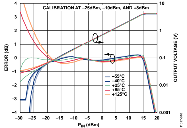
Figure 8. Conformance Error and Output Voltage (V OUT ) vs. RF Input Power (P IN ) for Various Temperatures at 1 GHz
