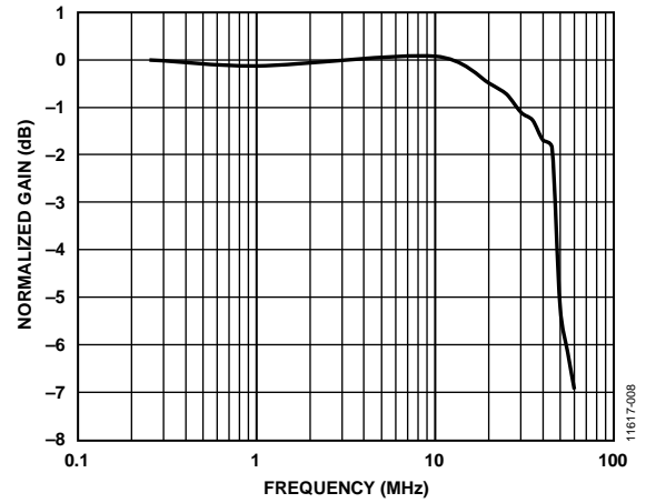
Figure 6. Envelope Bandwidth of V OUT vs. Frequency at P IN = -10 dBm and Modulation Depth = 10% (See Figure 36 in the Measurement Setups Section)
