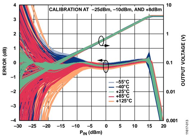
Figure 11. Distribution of Conformance Error with Respect to Output Voltage ( V_{out} ) at 25°C vs. RF Input Power ( P_{in} ) for Various Temperatures at 1 GHz
