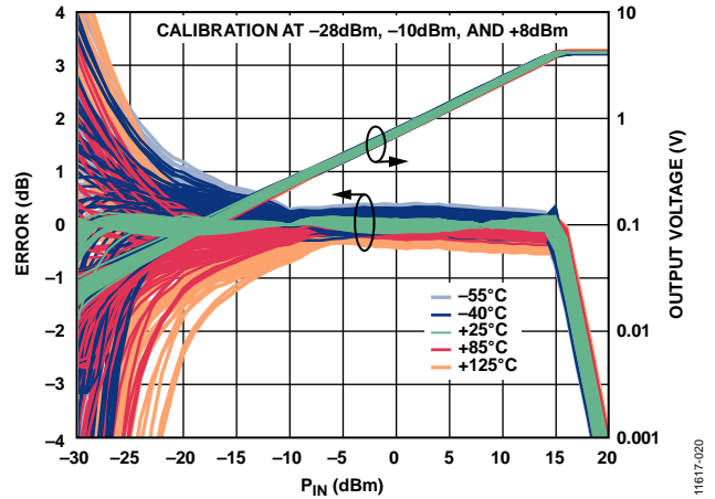
Figure 18. Distribution of Conformance Error with Respect to Output Voltage ( V_{OUT} ) at 25°C vs. RF Input Power ( P_{IN} ) for Various Temperatures at 20 GHz
