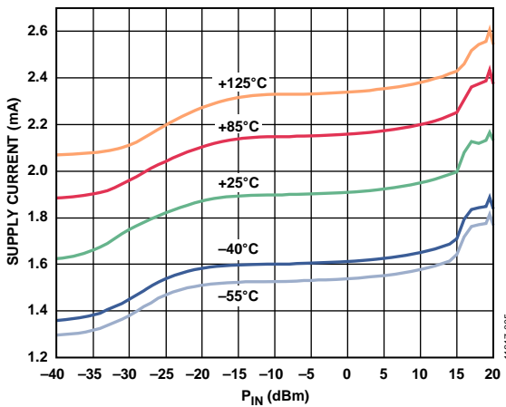
Figure 4. Supply Current vs. RF Input Power (P IN ) for Various Temperatures
