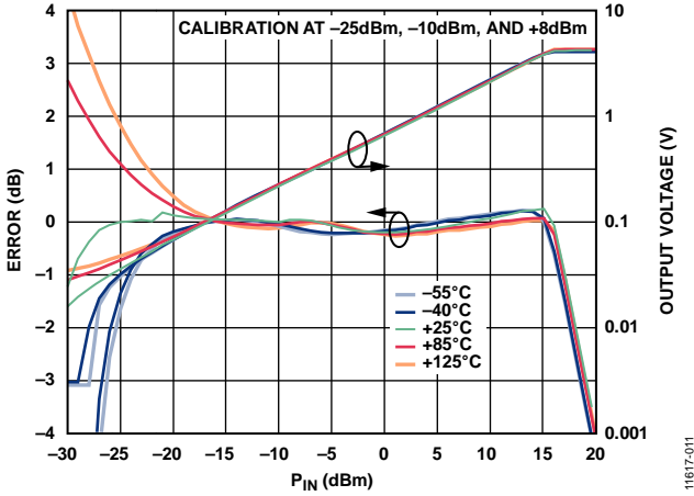
Figure 9. Conformance Error and Output Voltage ( V_{out} ) vs. RF Input Power ( P_{in} ) for Various Temperatures at 5 GHz
