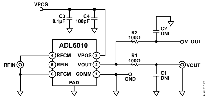
Figure 44. ADL6010 Evaluation Board Schematic
