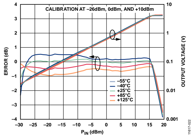
Figure 20. Conformance Error and Output Voltage ( V_{OUT} ) vs. RF Input Power ( P_{IN} ) for Various Temperatures at 30 GHz
