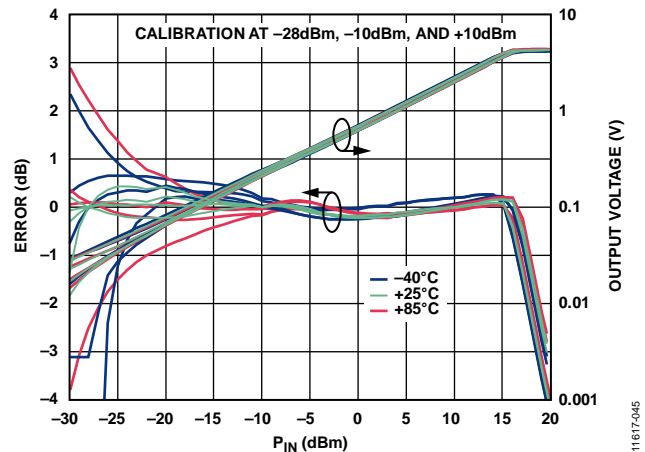
Figure 42. 10 GHz Conformance Error and Output Voltage vs. RF Input Power ( P_{IN} ) at +25°C, +85°C, and -40°C for Multiple Devices
