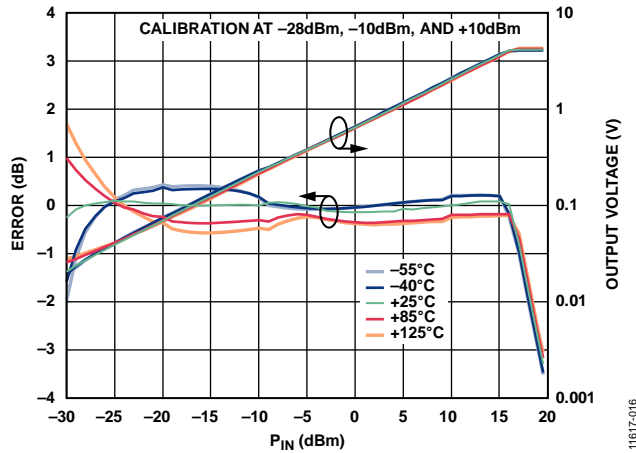
Figure 14. Conformance Error and Output Voltage ( V_{out} ) vs. RF Input Power ( P_{in} ) for Various Temperatures at 15 GHz
