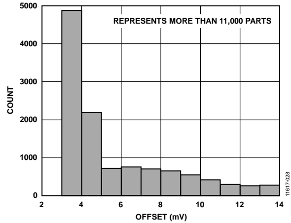
Figure 26. Distribution of V_{OUT} Offset with No Applied P_{IN} at 25°C
