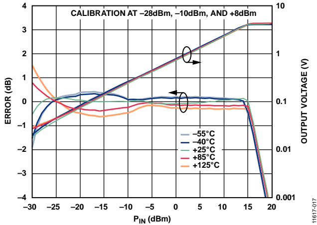
Figure 15. Conformance Error and Output Voltage ( V_{OUT} ) vs. RF Input Power ( P_{IN} ) for Various Temperatures at 20 GHz
