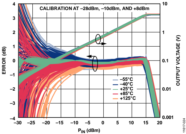
Figure 22. Distribution of Conformance Error with Respect to Output Voltage ( V_{OUT} ) at 25°C vs. RF Input Power ( P_{IN} ) for Various Temperatures at 25 GHz
