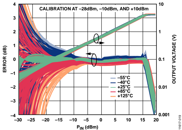
Figure 17. Distribution of Conformance Error with Respect to Output Voltage ( V_{OUT} ) at 25°C vs. RF Input Power ( P_{IN} ) for Various Temperatures at 15 GHz
