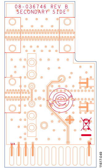
Figure 46. ADL6010 Evaluation Board Layout, Bottom Side
