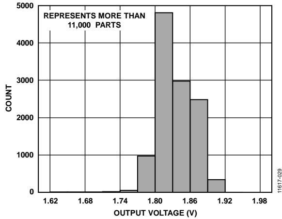
Figure 27. Output Voltage ( V_{OUT} ) Distribution, P_{IN} = 9 dBm at 12 GHz, 25°C
