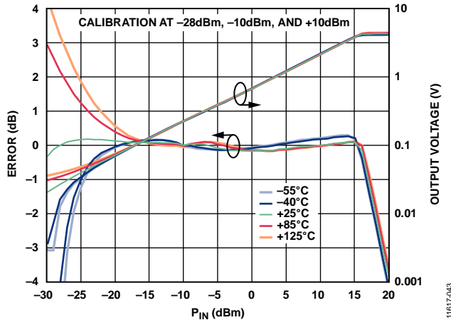
Figure 40. Conformance Error and Output Voltage vs. RF Input Power ( P_{IN} ) and Temperature (-55°C, -40°C, +25°C, +85°C, +125°C) at 10 GHz Using Three Point Calibration
