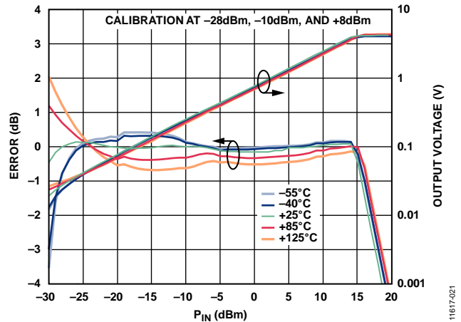
Figure 19. Conformance Error and Output Voltage ( V_{OUT} ) vs. RF Input Power ( P_{IN} ) for Various Temperatures at 25 GHz
