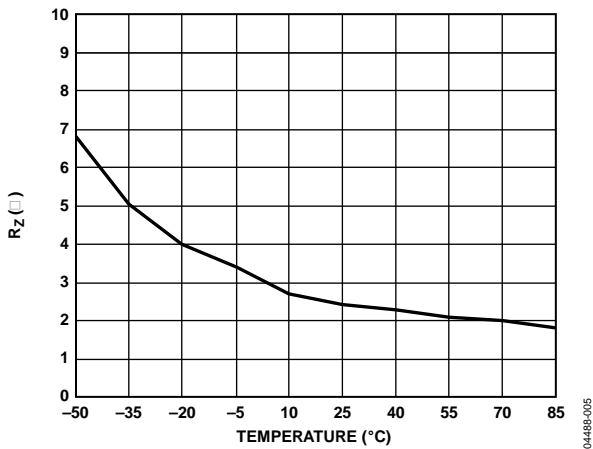
Figure 5. R Z (V IN Forward Voltage) vs. Temperature
