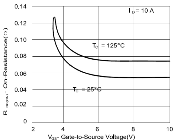
Figure 4: On-Resistance with Gate-to-source Voltage
