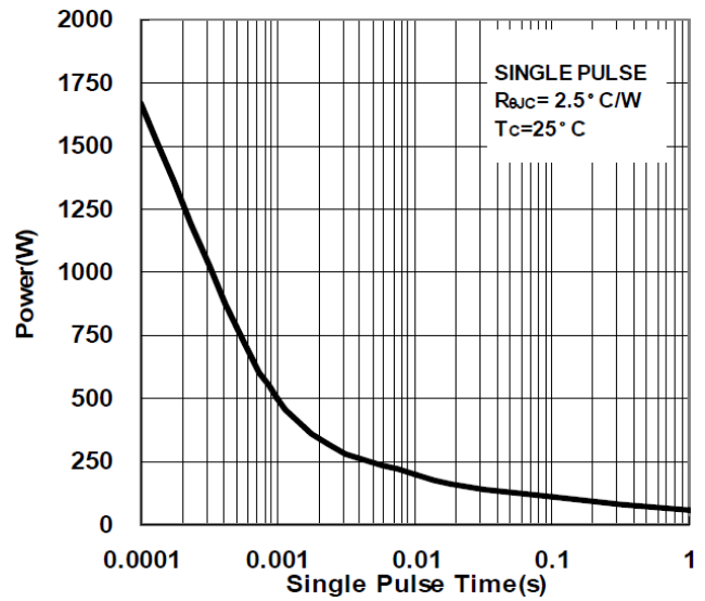
Figure 10: Pulse Maximum Power Dissipation
